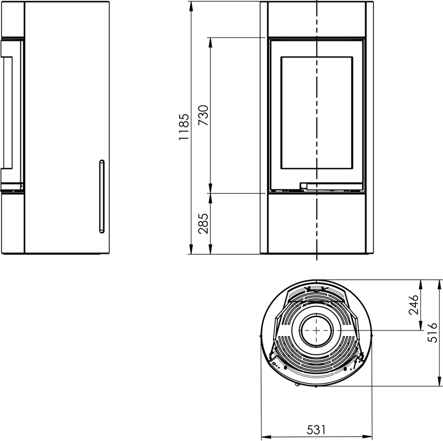
FIG 1b - Atlanta High / S-26R = mm
