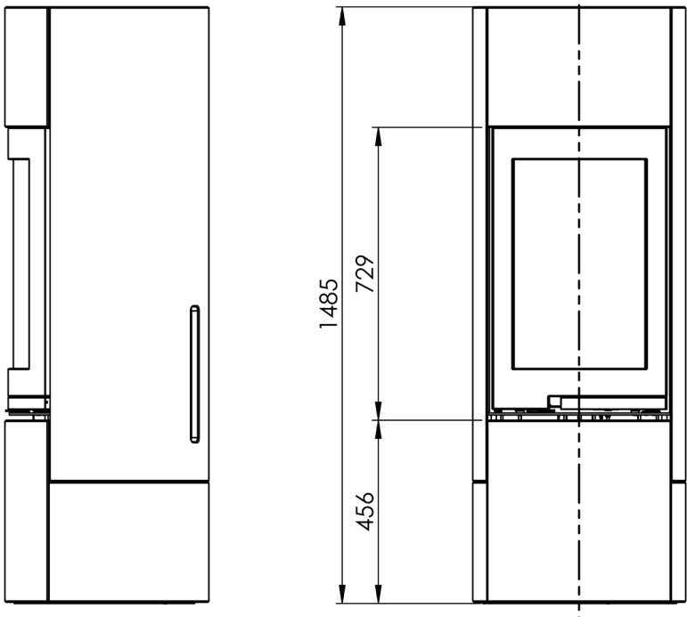
FIG 1b - Atlanta High / S-26R = mm
